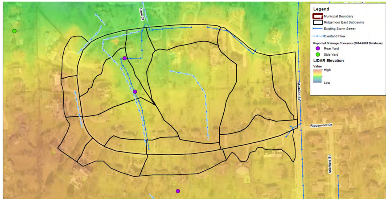
Figure 15. Ridgemoor East – Drainage Patterns
