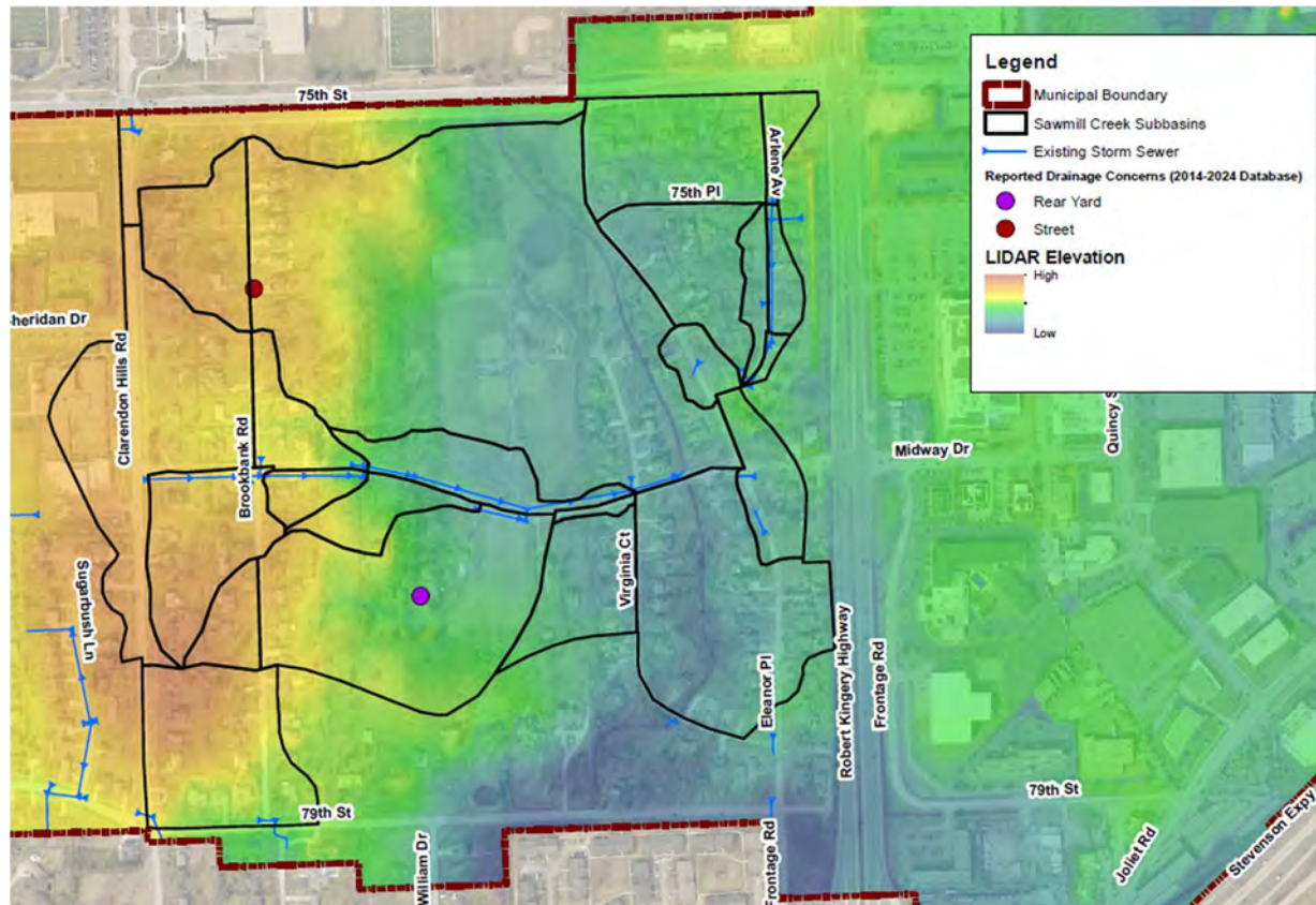
Figure 21. Sawmill Creek – Drainage Patterns and XPSWMM Routing
